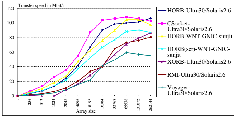
FIGURE 5. DOT Performance : byte array transfer with MTU = 1500
